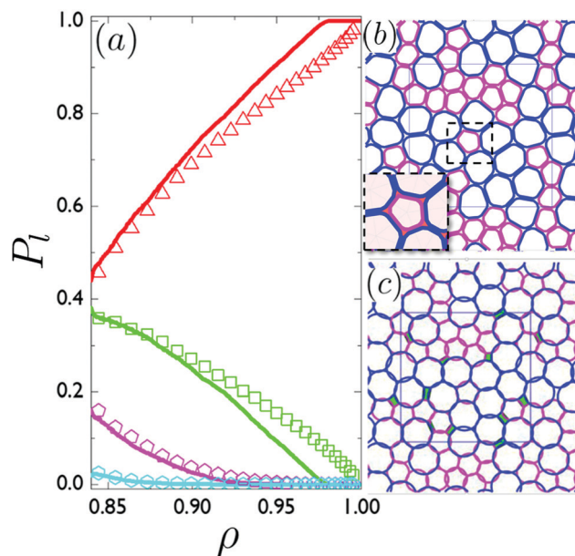
Fig. 7 (a) Probability P_l to have a void with l sides ( l = 3 (red), 4 (green), 5 (pink), and 6 (cyan)) for jammed packings as a function of \rho for the SP (symbols) and DP (lines) models. For both models, we studied ensembles of 500 jammed packings of N = 64 bidisperse particles. The void probability is normalized such that \sum_l P_l(\rho) = 1 . We also show
