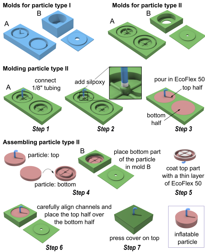
Fig. 2 Summary of the particle fabrication process. Each type of particle requires two sets of molds: one for molding the two halves (mold A) and one for assembling the two halves together (mold B). The components of the molds are 3D-printed out of Polyvinyl Lactic Acid (PLA). The blue (green) molds are used for type I (type II) particles. The fabrication process for both particle types is nearly identical, except for the use of slightly different mold designs. The seven-step fabrication process for type II particles is shown. The particles (pink) are molded from EcoFlex™ 50.
