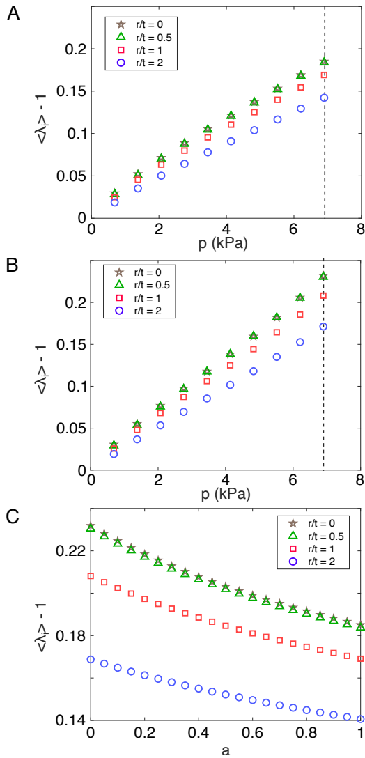
Fig. 5 The mean of the highest 1% of strains \langle \lambda_i \rangle - 1 plotted as a function of the inflation pressure p for type I particles with various r/t modeled using spring networks with (A) a = 1 and (B) 0. (C) Mean of the highest 1% of strains \langle \lambda_i \rangle - 1 plotted versus a at p = 6.89 kPa for type I particles with various r/t modeled using spring networks. The vertical dashed lines in (A) and (B) indicate the pressure used for the data in (C).
