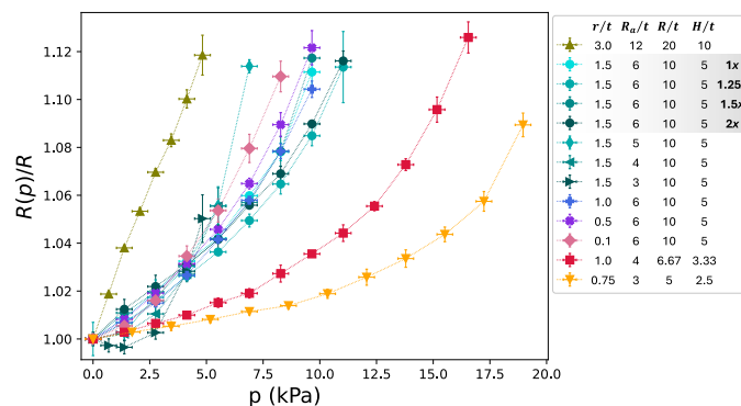
Fig. 8 Radius of the particle relative to the uninflated value, R(p)/R , as a function of the inflation pressure p for all type II particles studied in Fig. 7 with different combinations of r/t , H/t , R/t , and R_a/t . Each data point is an average over three samples measured three times each. The error bars indicate the standard deviation and the dotted lines are added as guides to the reader.
