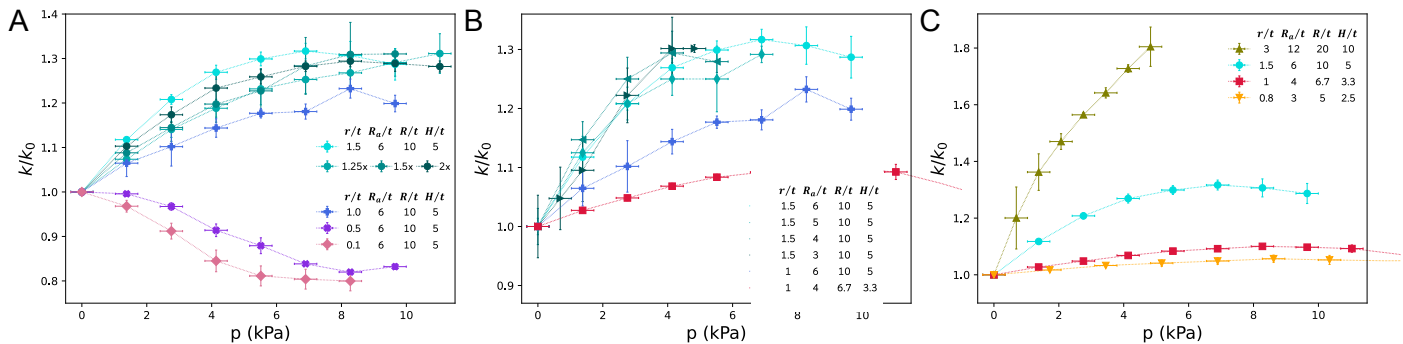
Fig. 7 Relative stiffness k/k_0 as a function of the inflation pressure p (in kPa) for type II particles with different combinations of r/t , H/t , R/t , and R_a/t . In (A), we show k(p) when (circles) all parameters are scaled proportionally at fixed r/t = 1.5 , as well as for (pluses) r/t = 1.0 , (crosses) 0.5, and (diamonds) 0.1 all at fixed R/t = 10 and R_a/t = 6 . In (B), we show (cyan) k(p) for R_a/t = 6 (circles), 5 (diamonds), 4 (leftward triangles), and 3 (rightward triangles) at fixed r/t = 1.5 and R/t = 10 . We also show k(p) when two ratios are varied: R_a/t = 6 and R/t = 10 (blue pluses) and R_a/t = 4 and R/t = 6.67 (red squares) both at fixed r/t = 1.0 . In (C), we show k(p) when all four ratios are varied. In all plots, each data point is an average over three samples measured three times each. The error bars indicate the standard deviation and the dotted lines are added as guides to the reader.
