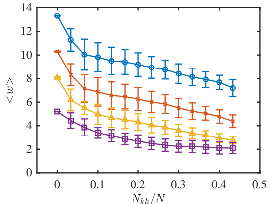
FIG. 19: The average maximum difference between adjacent eigenfrequencies \langle w \rangle of the mass-weighted dynamical matrix versus the number of contacts between the grains with knobs N_{kk}/N for a hexagonal packing with N_L = 21 and N_S = 9 and mass ratio m_L/m_S = 100 (circles), 20 (exes), 10 (triangles), and 5 (squares). The means and standard deviations (error bars) are obtained by averaging over 50 configurations in which the masses of the grains are chosen randomly as either m_L and m_S to yield a given N_{kk}/N .
