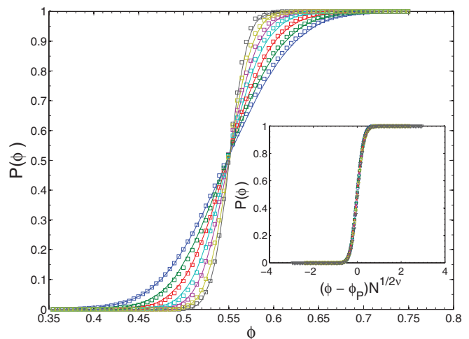
FIG. 2. (Color online) Percolation probability P(\phi) that the system possesses a system-spanning cluster (in either the x - or y -direction) immediately following a compression step \Delta\phi = 10^{-3} versus packing fraction \phi for N = 100, 200, 400, 800, 1600, 3200, and 6400 particles (from bottom left to right) averaged over 400 configurations for bidisperse (lines) and monodisperse (squares) particle size distributions. Inset: Same as the main figure for the bidisperse systems except the horizontal axis is scaled by (\phi - \phi_p)N^{1/2\nu} , where \phi_p = 0.549 \pm 0.001 and \nu = 1.68 \pm 0.08 .
